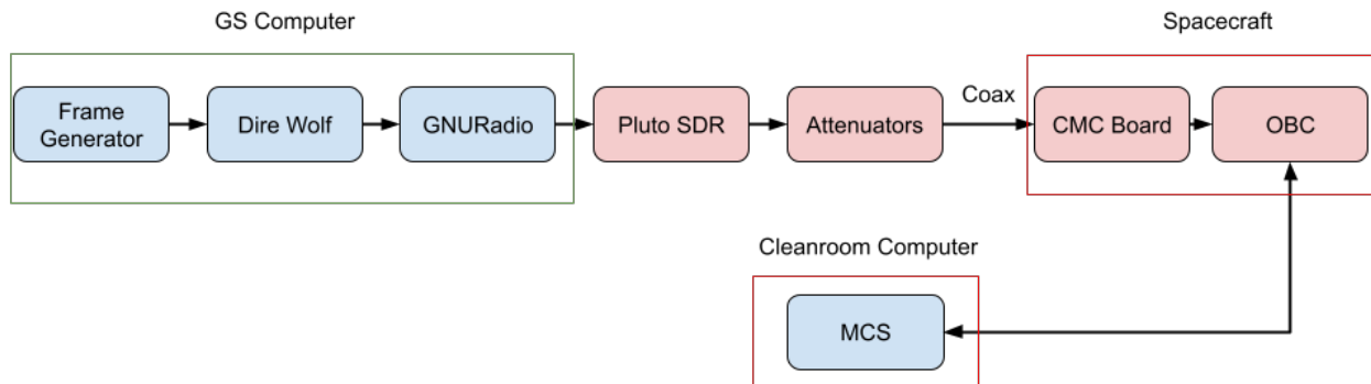
Fig. 4 The setup used for the BER test for the EIRSAT-1 uplink. The boxes in blue denote software components, with the red boxes denoting hardware components. A coaxial cable was used to connect the attenuators to the CMC board of the spacecraft.
